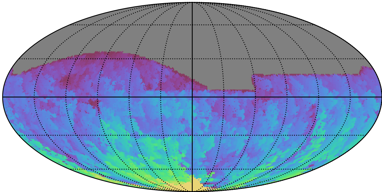
ddf_acor_sf15_lsf40_lsr10_v3.4_10yrs All sky g band: Max HA
