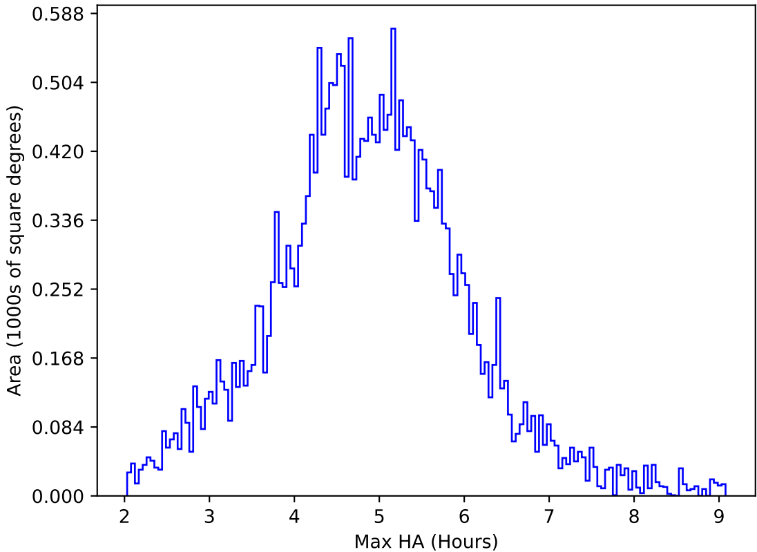
ddf_acor_sf15_lsf40_lsr10_v3.4_10yrs All sky all bands: Max HA
