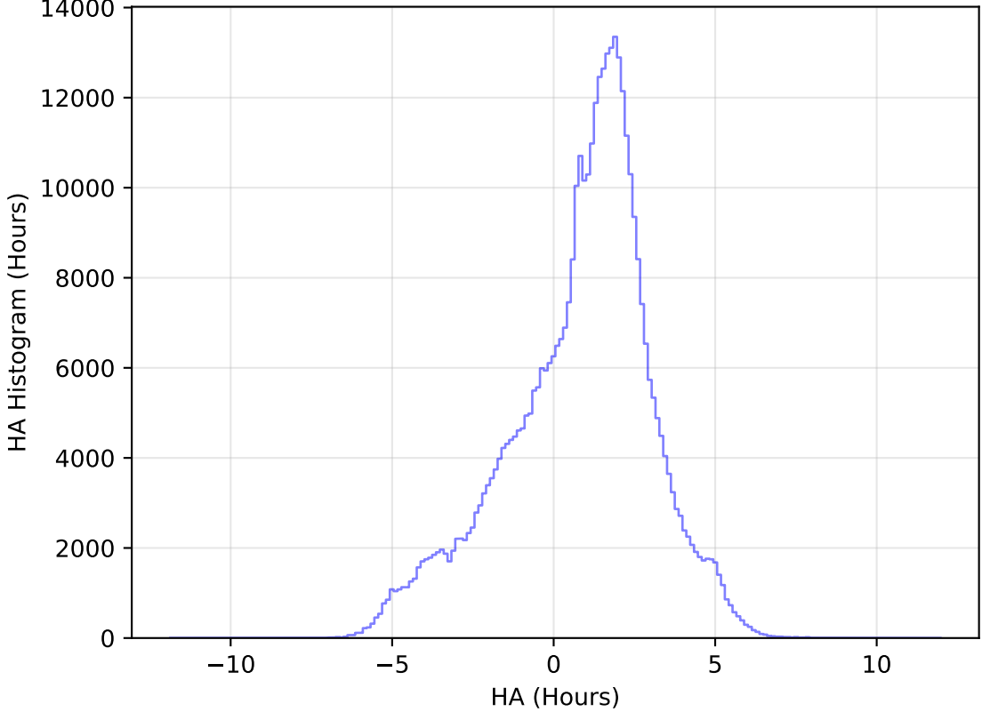
ddf_acor_sf15_lsf40_lsr10_v3.4_10yrs WFD z band: HA Histogram
