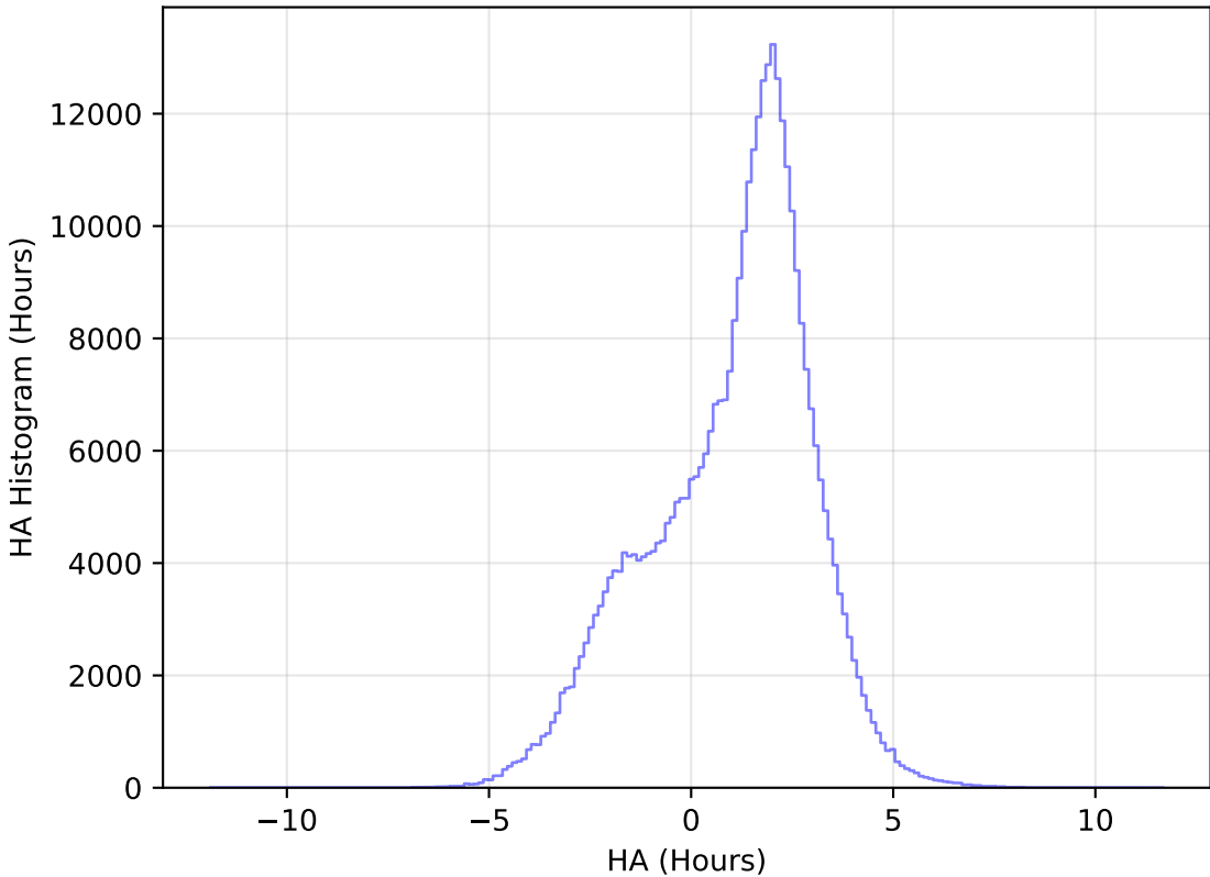
ddf_acor_sf15_lsf40_lsr10_v3.4_10yrs WFD y band: HA Histogram
