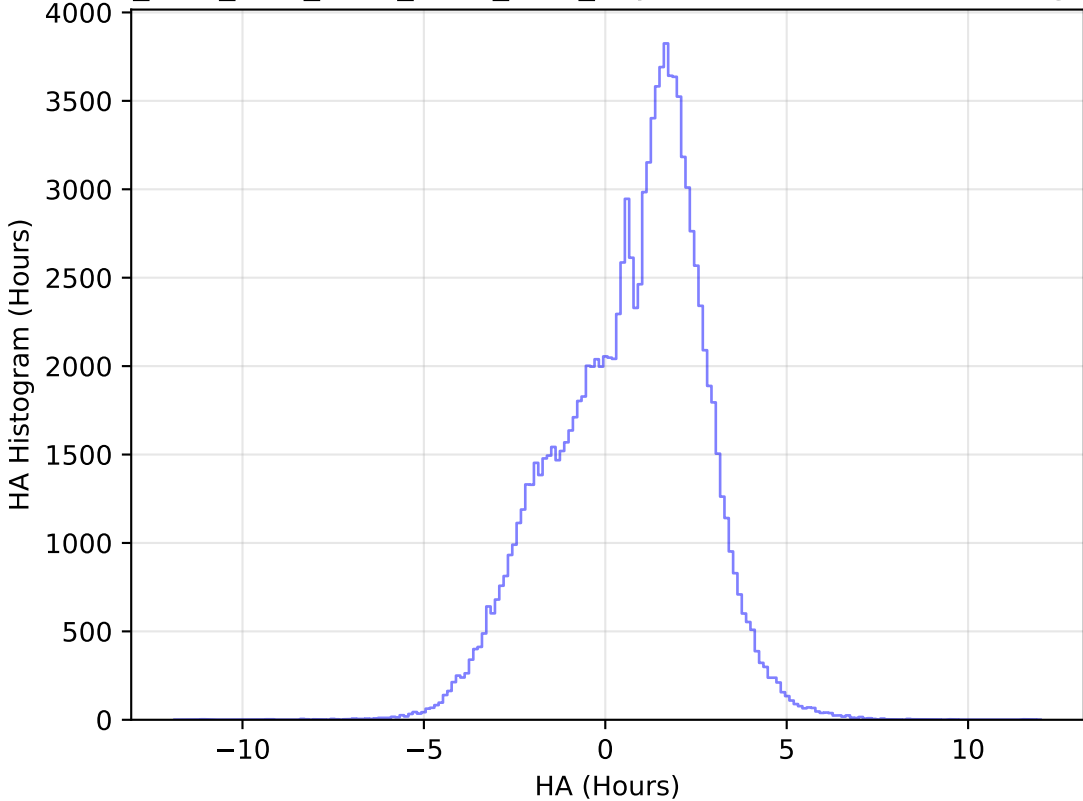
ddf_acor_sf15_lsf40_lsr10_v3.4_10yrs WFD u band: HA Histogram
