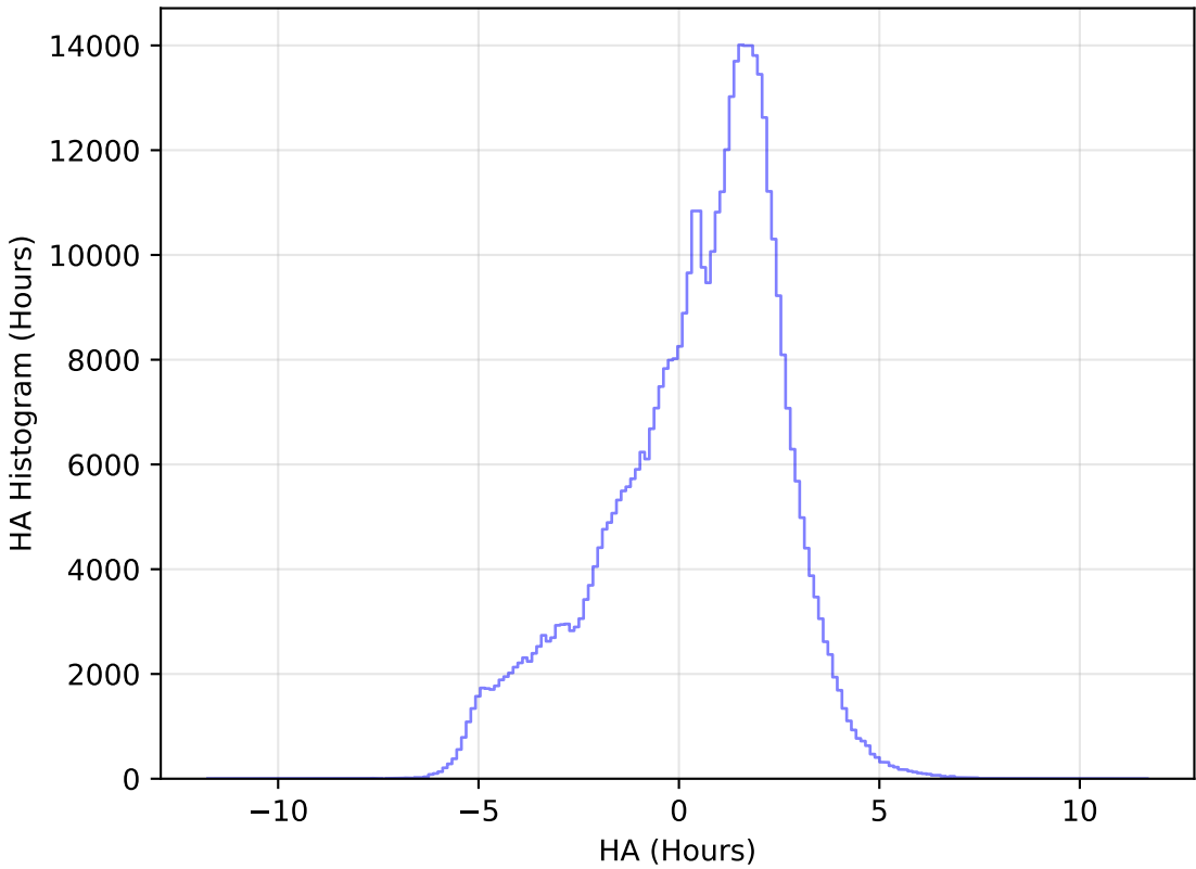
ddf_acor_sf15_lsf40_lsr10_v3.4_10yrs WFD r band: HA Histogram
