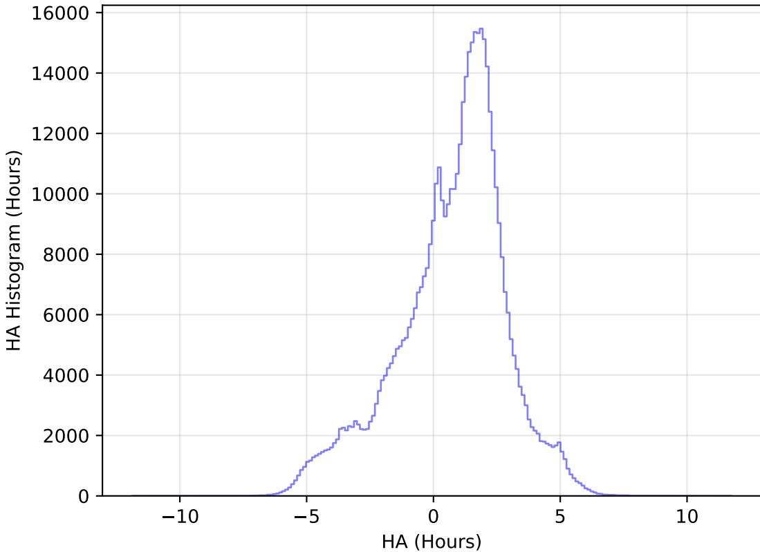
ddf_acor_sf15_lsf40_lsr10_v3.4_10yrs WFD i band: HA Histogram
