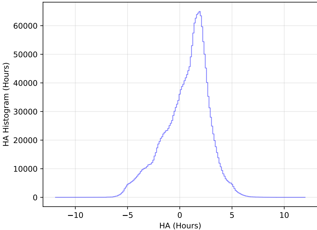
ddf_acor_sf15_lsf40_lsr10_v3.4_10yrs WFD all bands: HA Histogram
