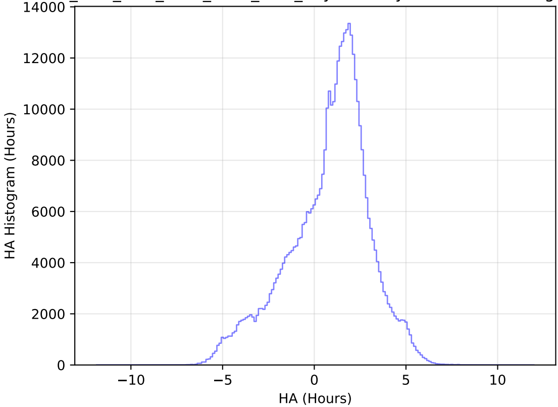
ddf_acor_sf15_lsf40_lsr10_v3.4_10yrs All sky z band: HA Histogram
