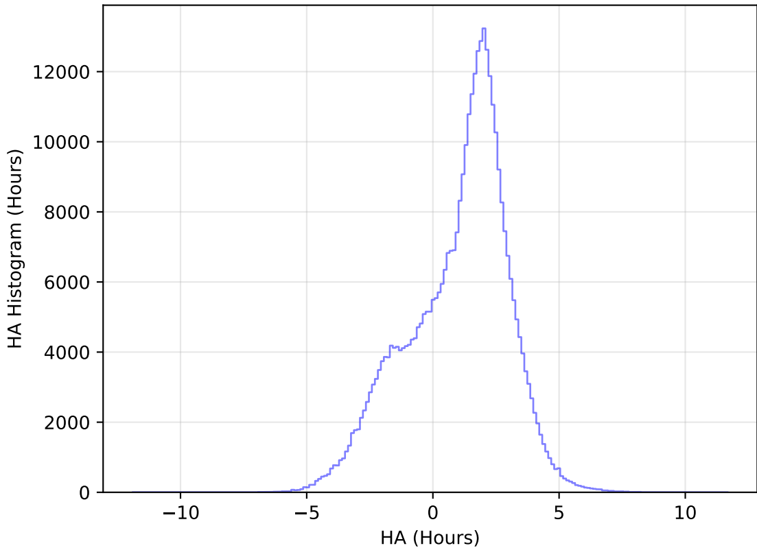
ddf_acor_sf15_lsf40_lsr10_v3.4_10yrs All sky y band: HA Histogram
