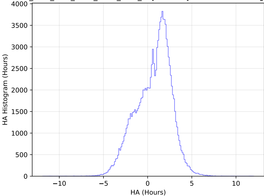
ddf_acor_sf15_lsf40_lsr10_v3.4_10yrs All sky u band: HA Histogram
