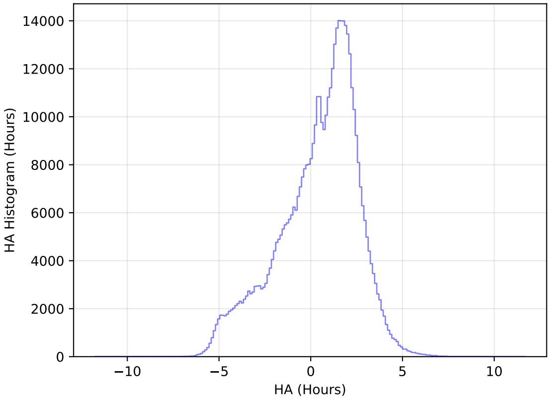
ddf_acor_sf15_lsf40_lsr10_v3.4_10yrs All sky r band: HA Histogram
