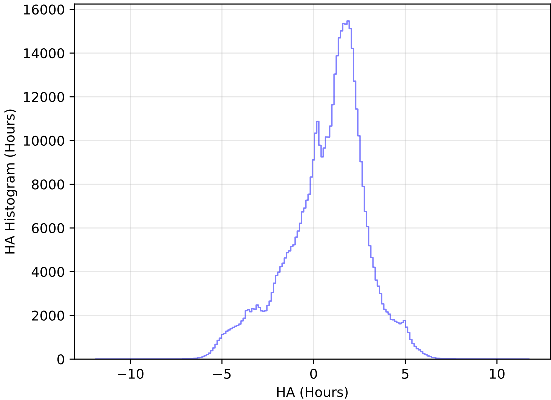
ddf_acor_sf15_lsf40_lsr10_v3.4_10yrs All sky i band: HA Histogram
