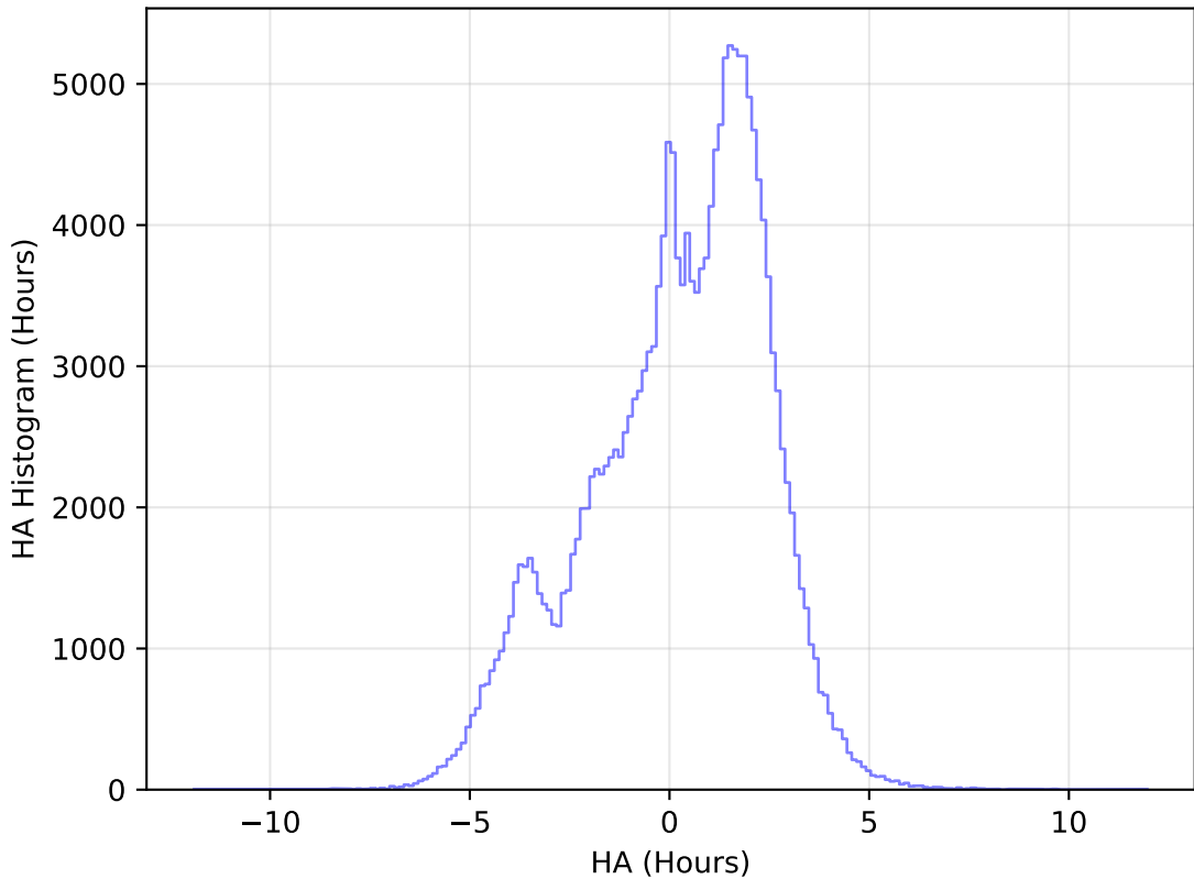
ddf_acor_sf15_lsf40_lsr10_v3.4_10yrs All sky g band: HA Histogram
