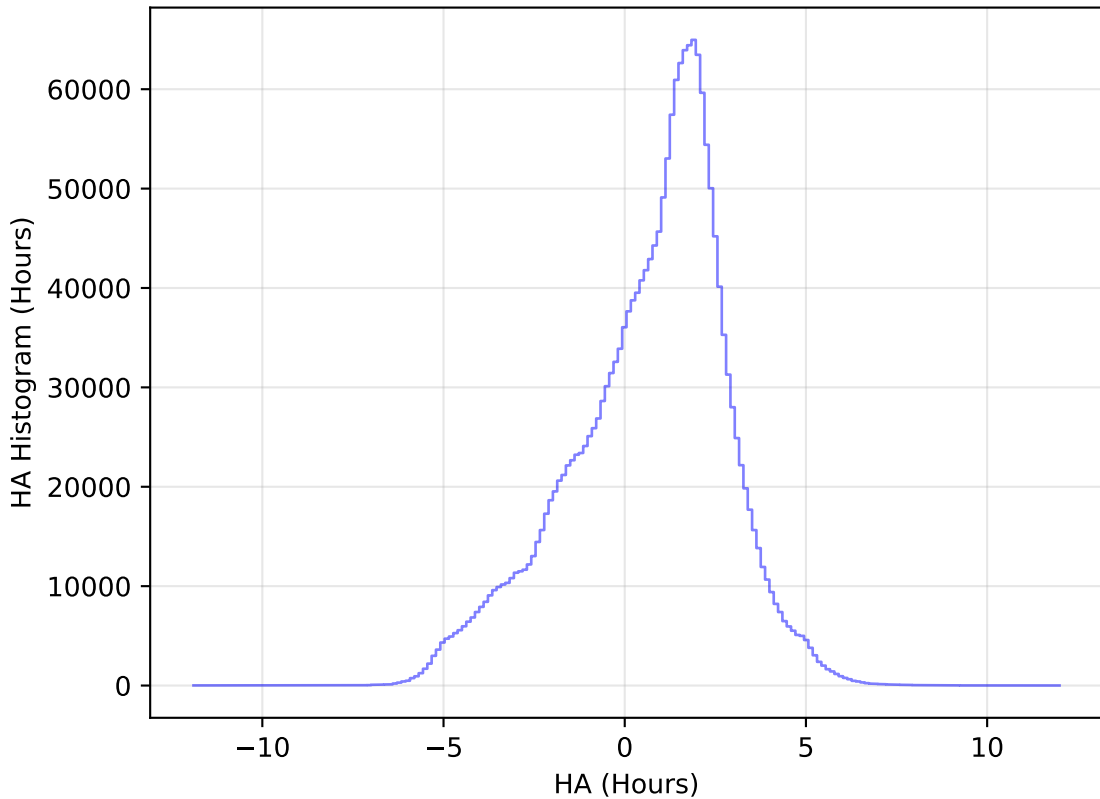
ddf_acor_sf15_lsf40_lsr10_v3.4_10yrs All sky all bands: HA Histogram
