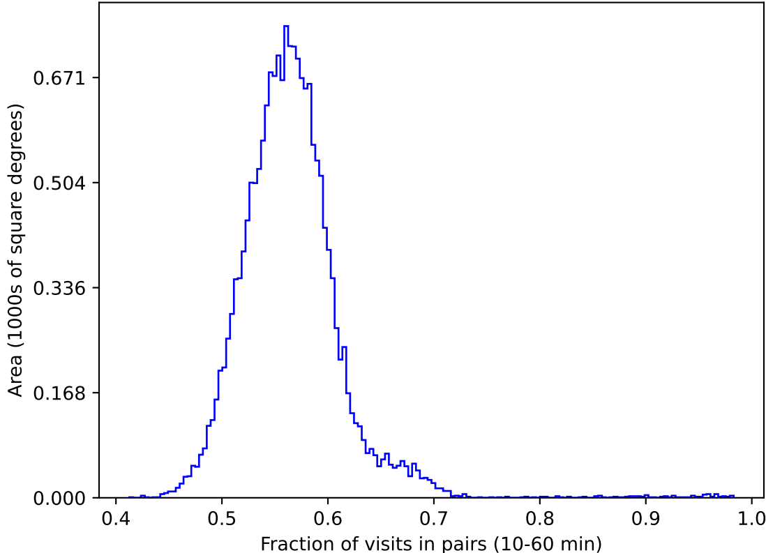
ddf_acor_sf15_ls40_lsr10_v3.4_10yrs gri WFD: Fraction of visits in pairs (10-60 min)
