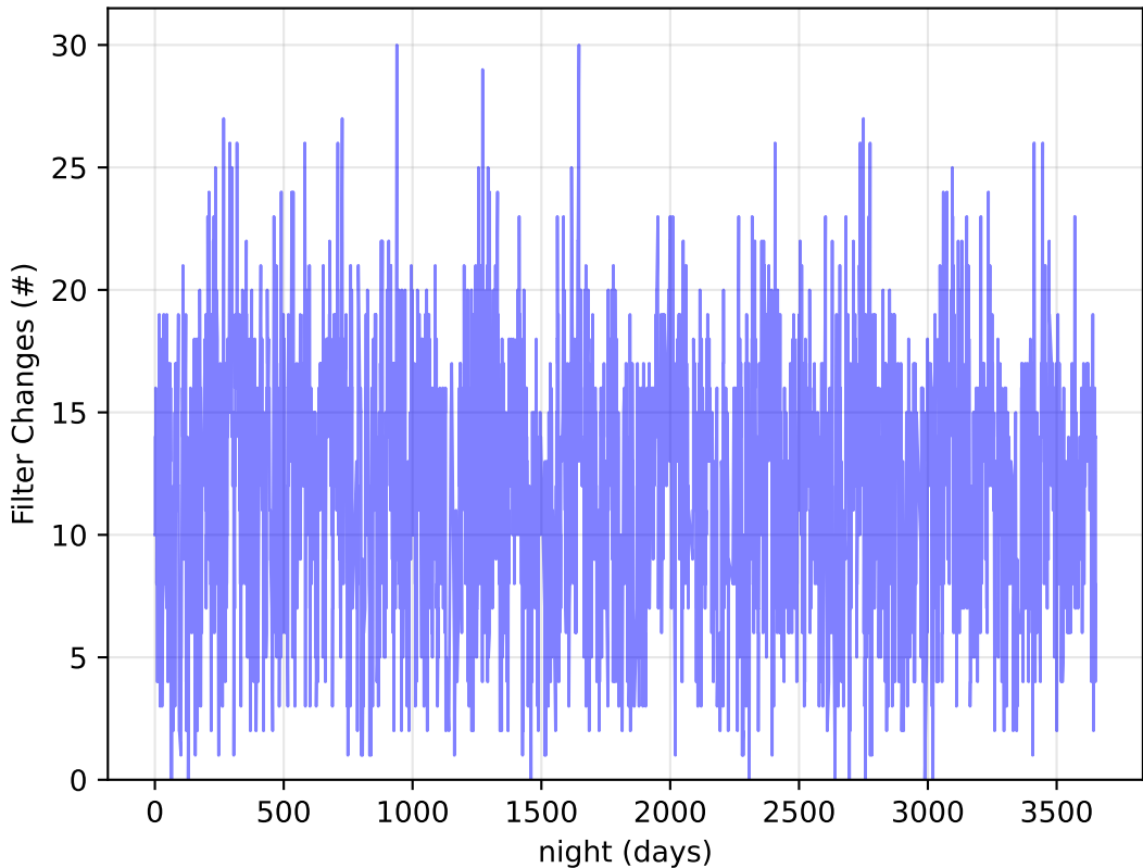
ddf_acor_sf15_lsf40_lsr10_v3.4_10yrs Per Night: Filter Changes
