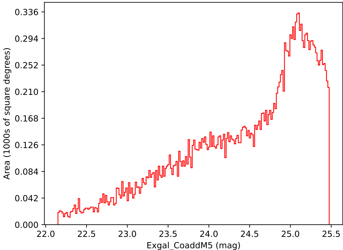
ddf_acor_sf15_lsf40_lsr10_v3.4_10yrs Yr 3-4 i band: Exgal_CoaddM5
