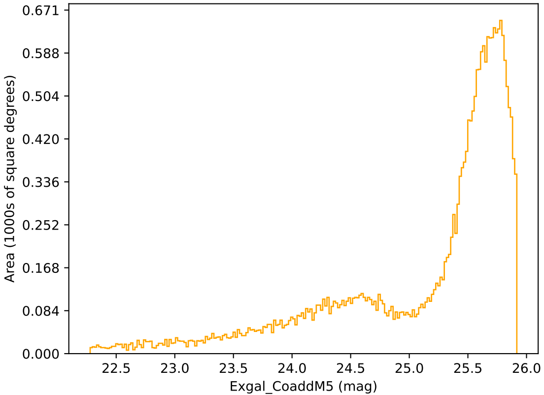
ddf_acor_sf15_lsf40_lsr10_v3.4_10yrs Yr 1 r band: Exgal_CoaddM5
