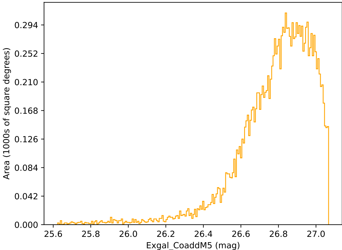
ddf_acor_sf15_lsf40_lsr10_v3.4_10yrs WFD r band: Exgal_CoaddM5
