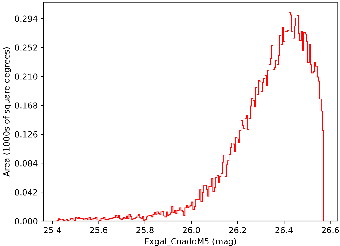
ddf_acor_sf15_lsf40_lsr10_v3.4_10yrs WFD i band: Exgal_CoaddM5
