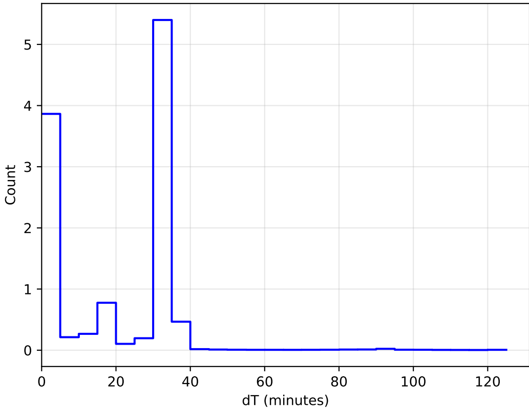
ddf_acor_sf15_lsf40_lsr10_v3.4_10yrs WFD: DeltaT Histogram 1e6
