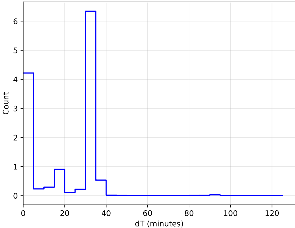
ddf_acor_sf15_lsf40_lsr10_v3.4_10yrs All sky: DeltaT Histogram
