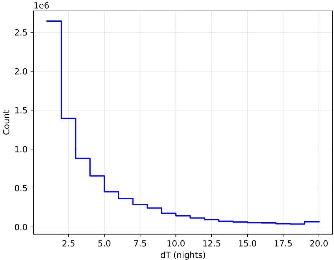
ddf_acor_sf15_lsf40_lsr10_v3.4_10yrs WFD all bands: DeltaNight Histogram
