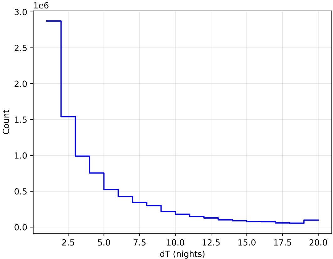
ddf_acor_sf15_lsf40_lsr10_v3.4_10yrs All sky all bands: DeltaNight Histogram
