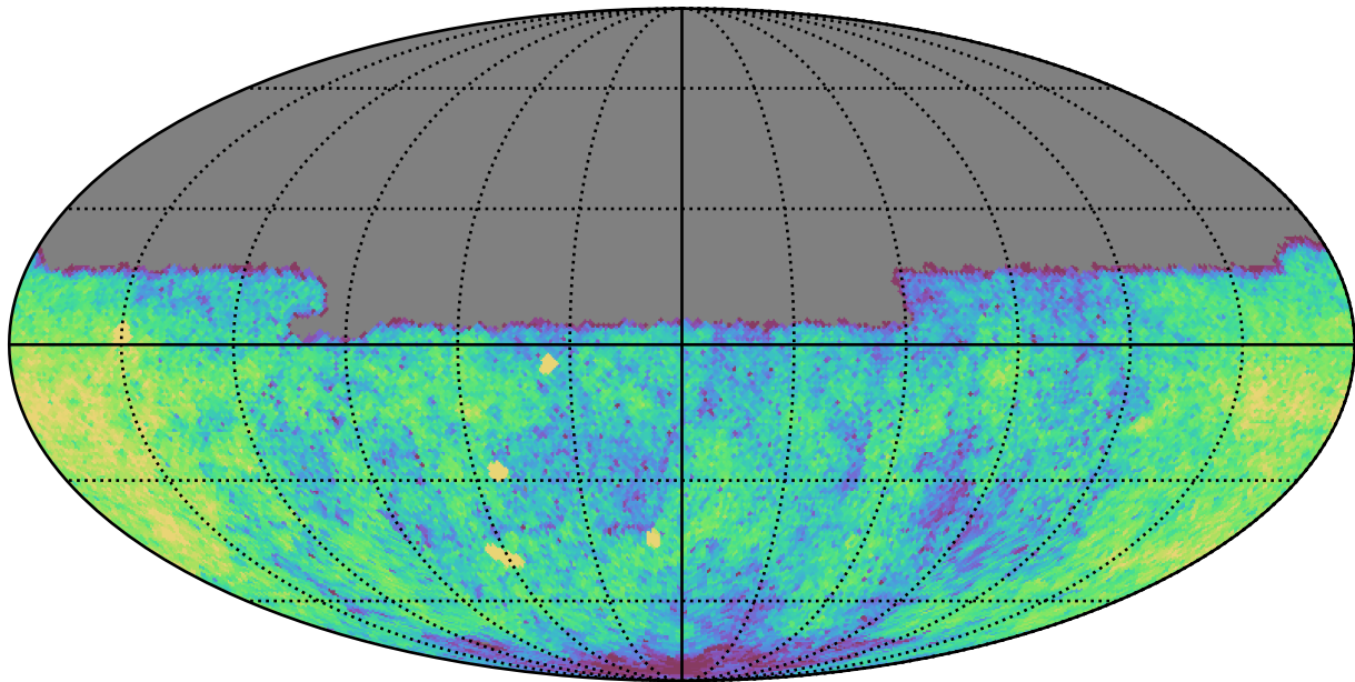
ddf_acor_sf15_lsf40_lsr10_v3.4_10yrs Yr 1 u band: CoaddM5
