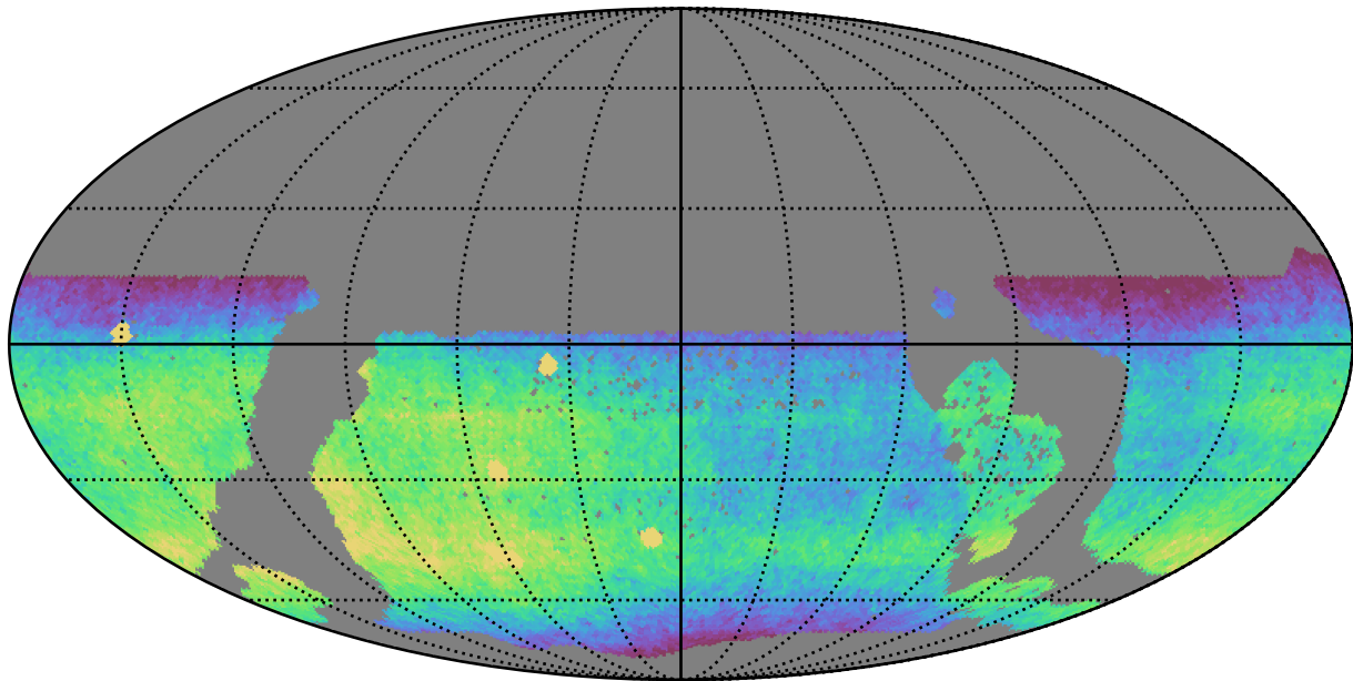
ddf_acor_sf15_lsf40_lsr10_v3.4_10yrs WFD r band: CoaddM5
