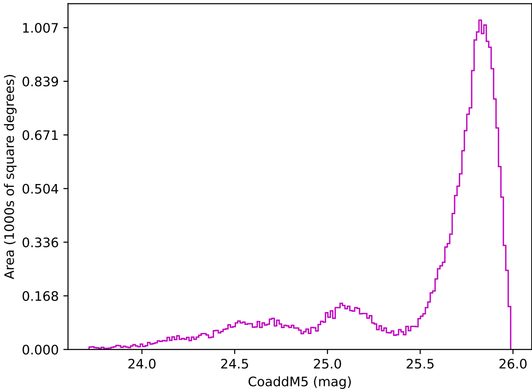
ddf_acor_sf15_lsf40_lsr10_v3.4_10yrs All sky z band: CoaddM5
