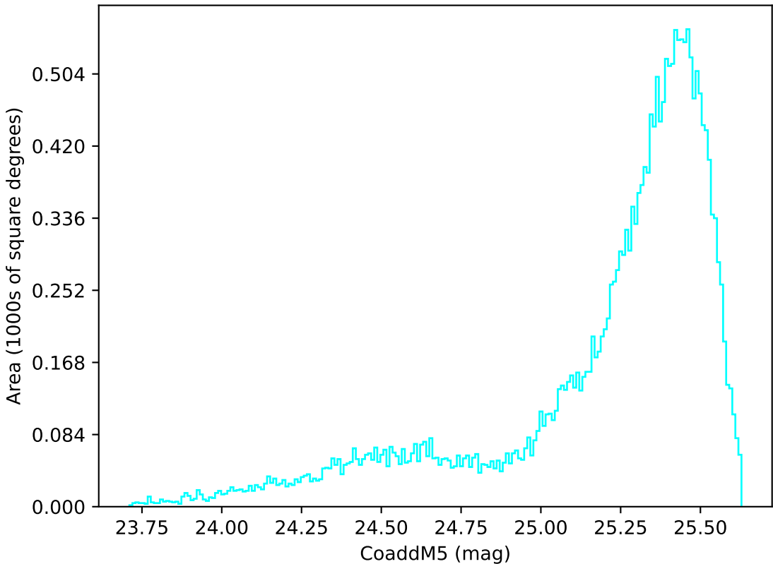
ddf_acor_sf15_lsf40_lsr10_v3.4_10yrs All sky u band: CoaddM5
