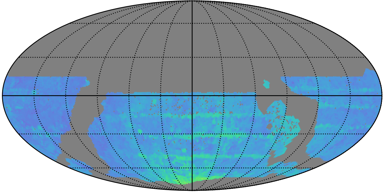
ddf_acor_sf15_lsf40_lsr10_v3.4_10yrs WFD z band: 80thPercentile Season Length
