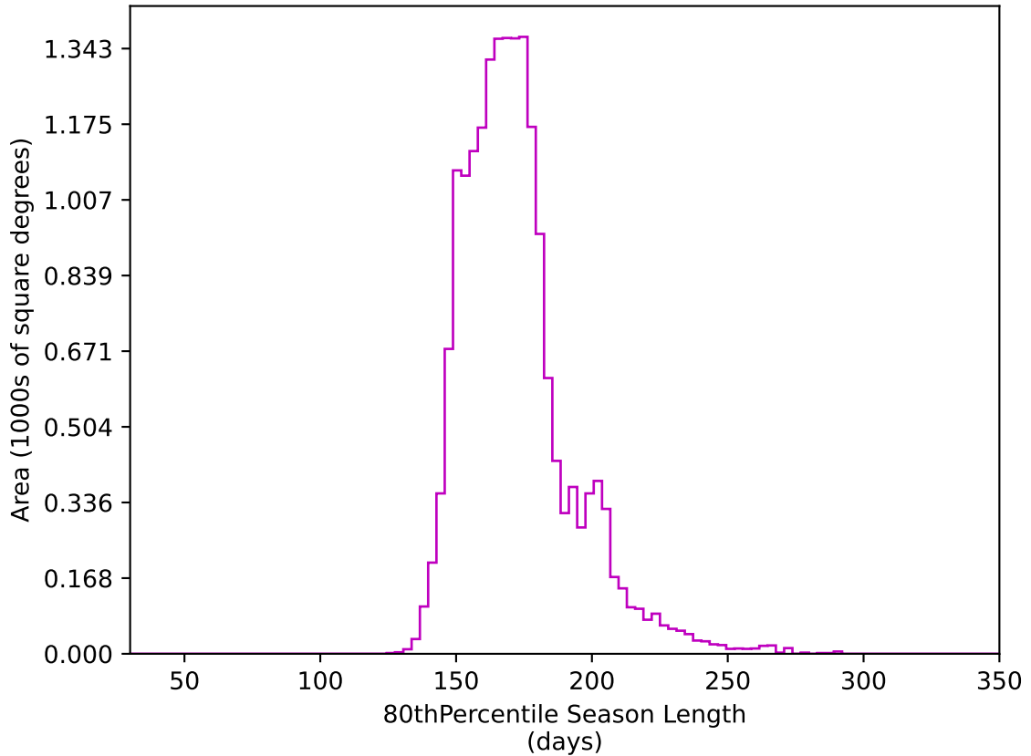
ddf_acor_sf15_lsf40_lsr10_v3.4_10yrs WFD z band: 80thPercentile Season Length
