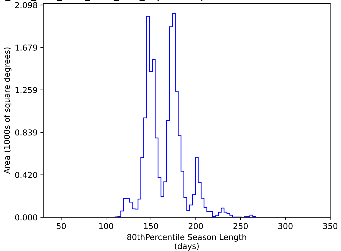
ddf_acor_sf15_lsf40_lsr10_v3.4_10yrs WFD y band: 80thPercentile Season Length
