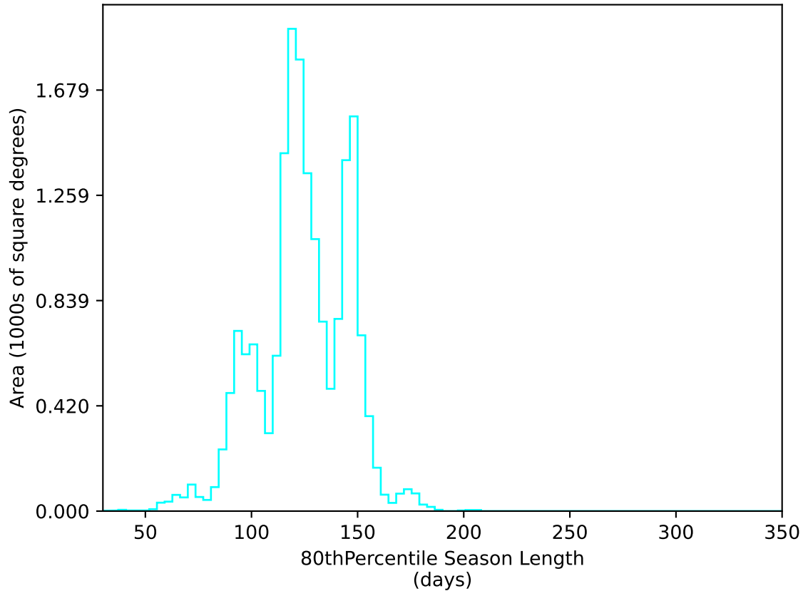
ddf_acor_sf15_lsf40_lsr10_v3.4_10yrs WFD u band: 80thPercentile Season Length
