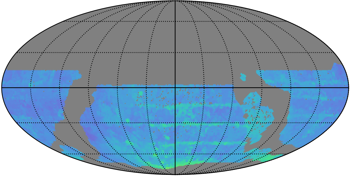
ddf_acor_sf15_lsf40_lsr10_v3.4_10yrs WFD r band: 80thPercentile Season Length
