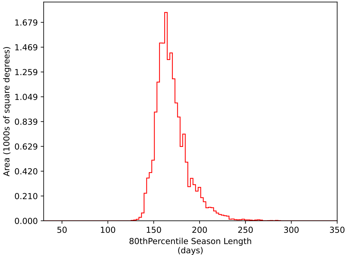
ddf_acor_sf15_lsf40_lsr10_v3.4_10yrs WFD i band: 80thPercentile Season Length
