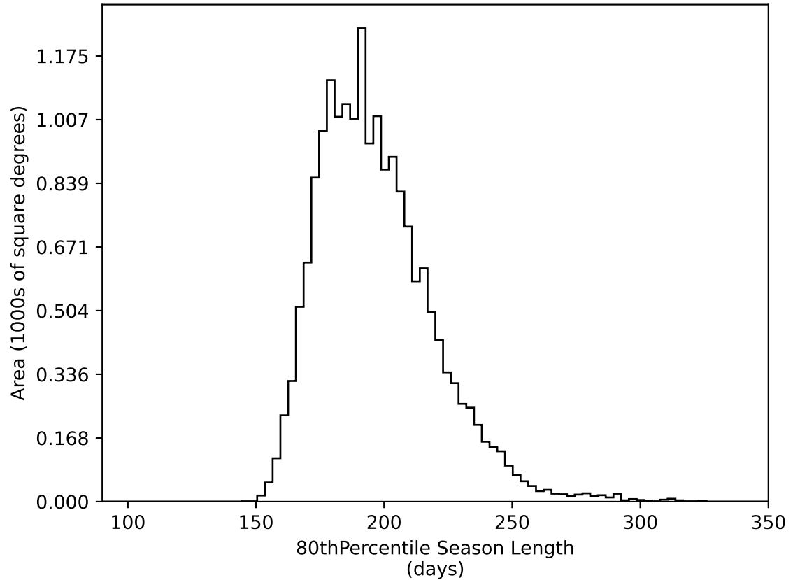
ddf_acor_sf15_lsf40_lsr10_v3.4_10yrs WFD all bands: 80thPercentile Season Length
