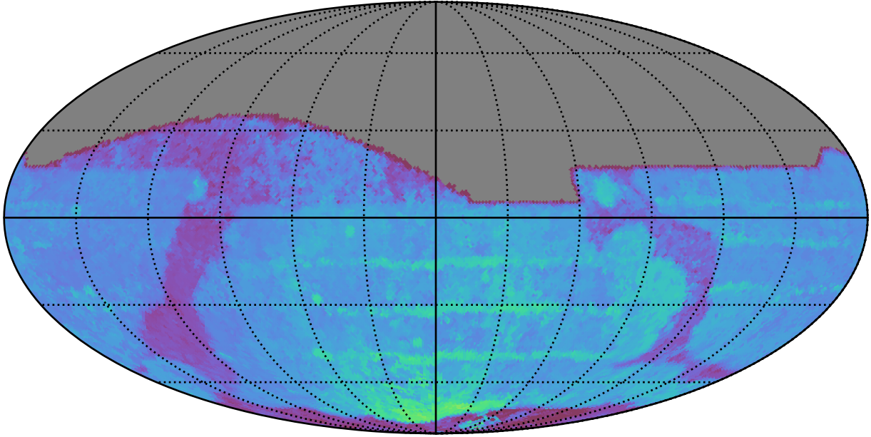
ddf_acor_sf15_lsf40_lsr10_v3.4_10yrs All sky z band: 80thPercentile Season Length
