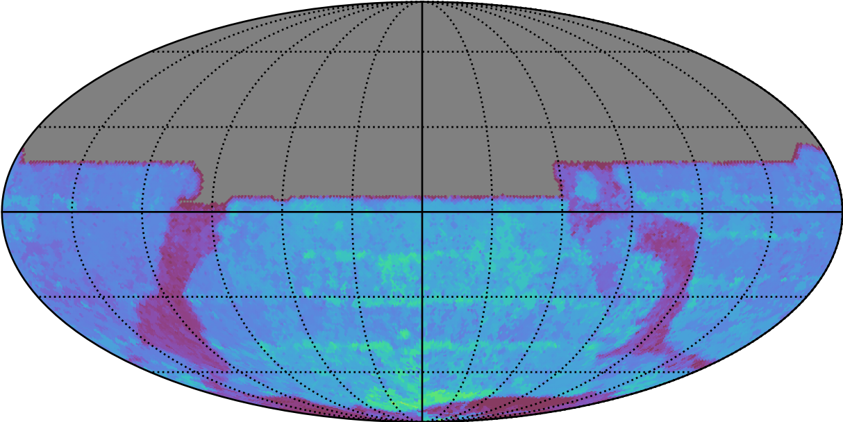
ddf_acor_sf15_lsf40_lsr10_v3.4_10yrs All sky y band: 80thPercentile Season Length
