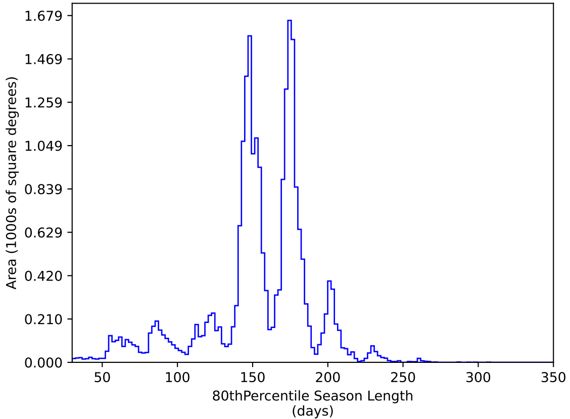
ddf_acor_sf15_lsf40_lsr10_v3.4_10yrs All sky y band: 80thPercentile Season Length
