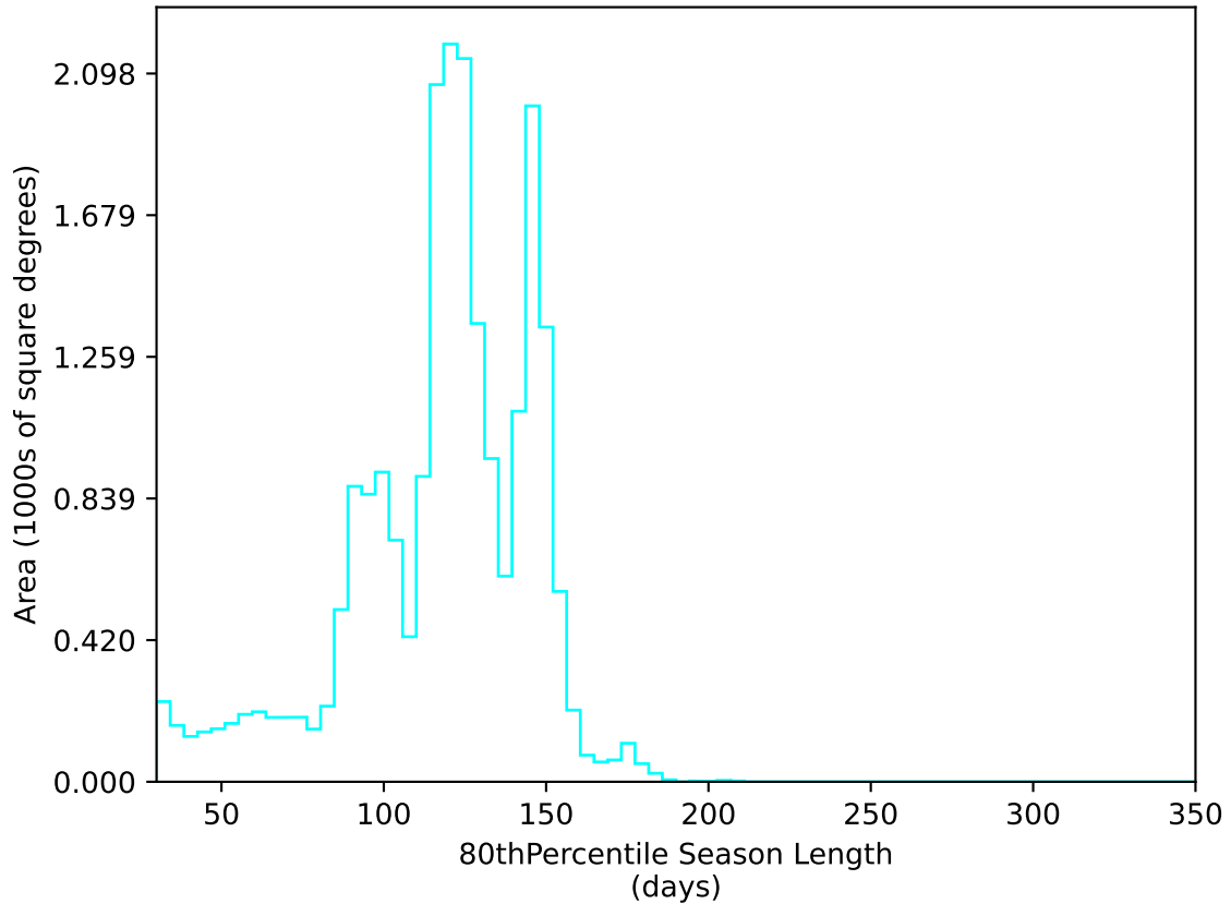
ddf_acor_sf15_lsf40_lsr10_v3.4_10yrs All sky u band: 80thPercentile Season Length
