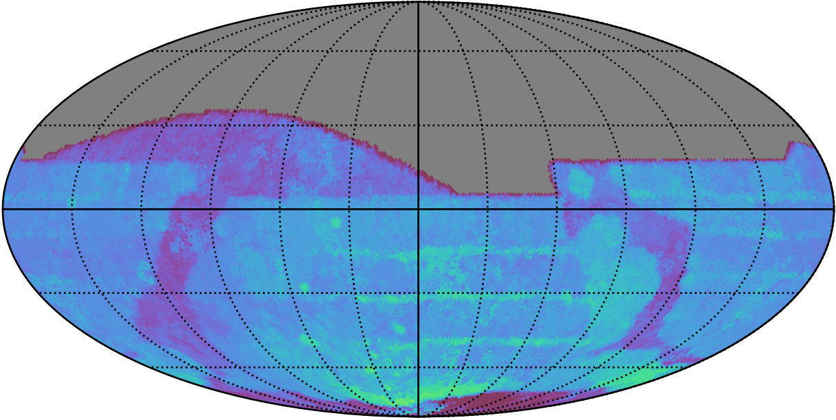
ddf_acor_sf15_lsf40_lsr10_v3.4_10yrs All sky r band: 80thPercentile Season Length
