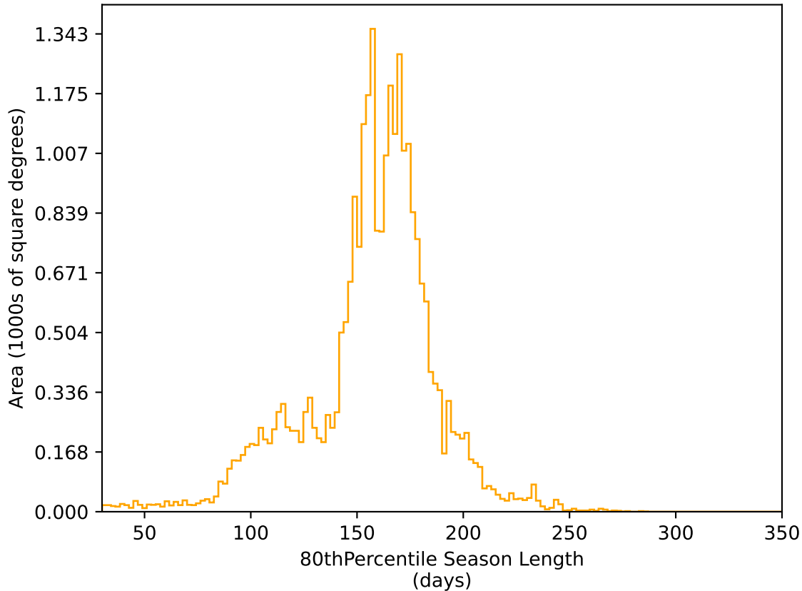
ddf_acor_sf15_lsf40_lsr10_v3.4_10yrs All sky r band: 80thPercentile Season Length
