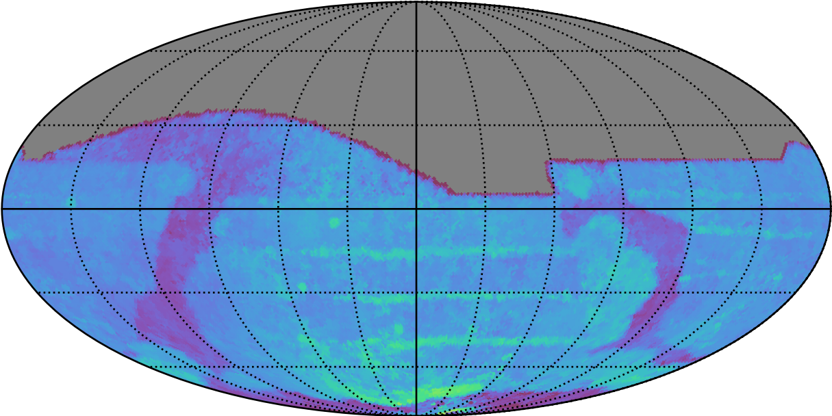
ddf_acor_sf15_lsf40_lsr10_v3.4_10yrs All sky i band: 80thPercentile Season Length
