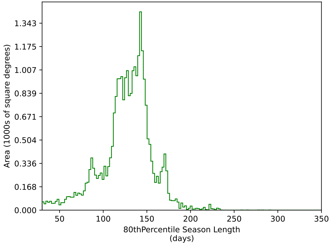
ddf_acor_sf15_lsf40_lsr10_v3.4_10yrs All sky g band: 80thPercentile Season Length
