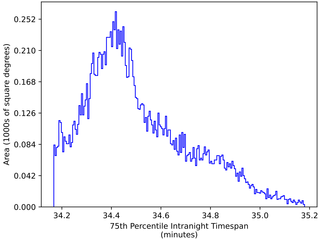
ddf_acor_sf15_lsf40_lsr10_v3.4_10yrs WFD zy bands: 75th Percentile Intranight Timespan
