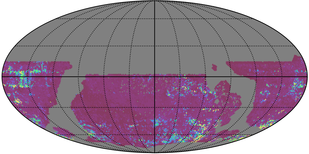
ddf_acor_sf15_lsf40_lsr10_v3.4_10yrs WFD z band: 75th Percentile Intranight Timespan
