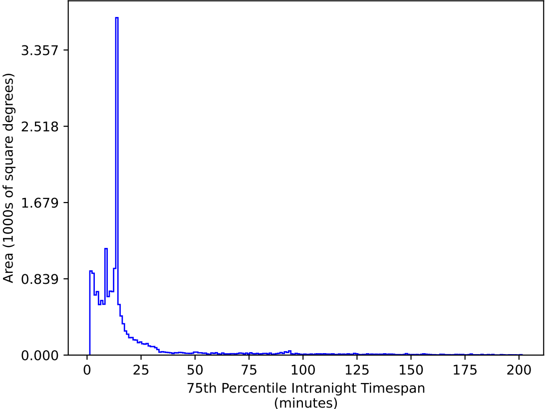
ddf_acor_sf15_lsf40_lsr10_v3.4_10yrs WFD z band: 75th Percentile Intranight Timespan
