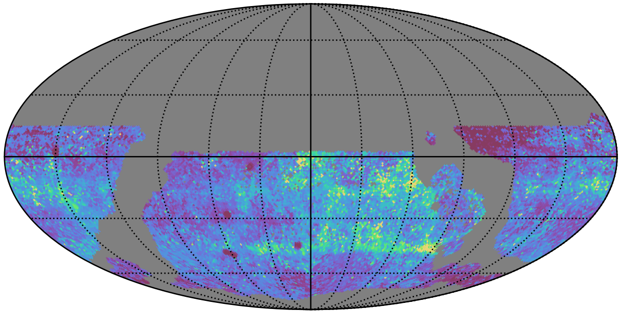
ddf_acor_sf15_lsf40_lsr10_v3.4_10yrs WFD y band: 75th Percentile Intranight Timespan
