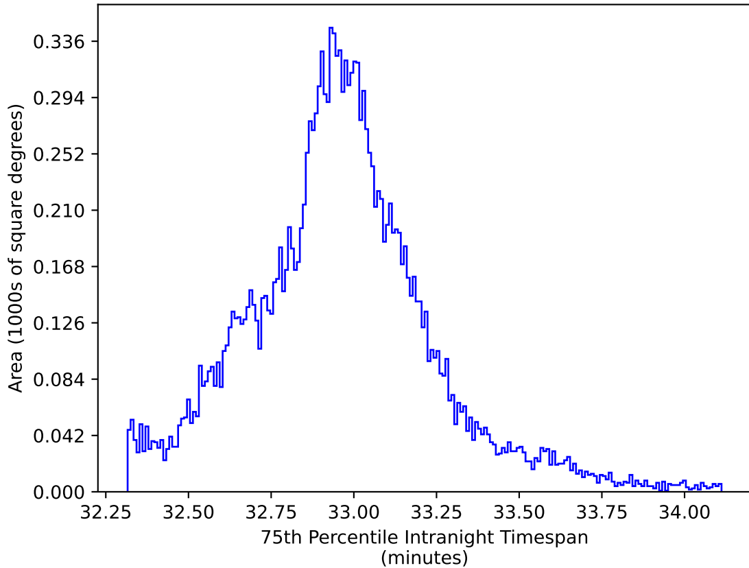
ddf_acor_sf15_lsf40_lsr10_v3.4_10yrs WFD y band: 75th Percentile Intranight Timespan
