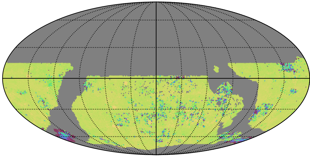
ddf_acor_sf15_lsf40_lsr10_v3.4_10yrs WFD ug bands: 75th Percentile Intranight Timespan
